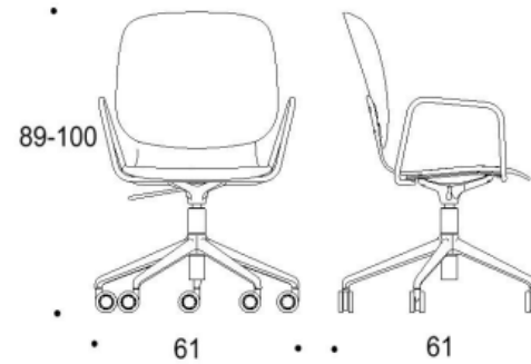
Two-part high back with armrest
